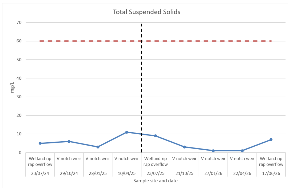
Figure 12 Total suspended solids- Bypass Creek V-notch weir and Wetland Rip Rap Overflow surface water sampling sites
