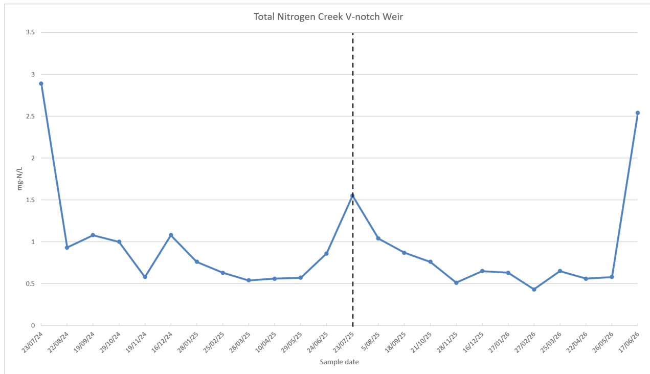
Figure 15 Nitrogen (Total) - Bypass Creek V-notch Weir
