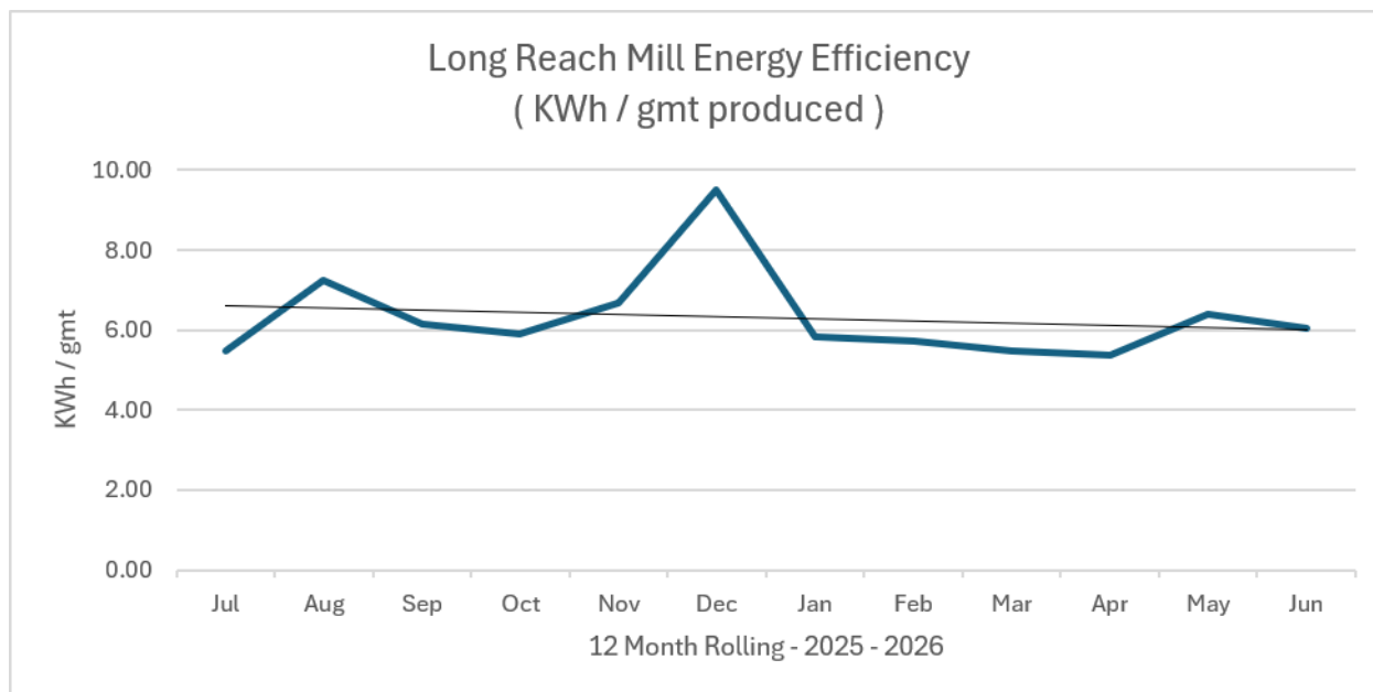
Figure 5 Energy consumption per gmt produced, 2025-2026 reporting period
