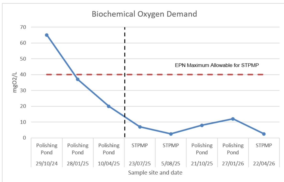
Figure 9 BOD levels (mg O 2 /L) Long Reach South Mill STPMP and Polishing Pond
