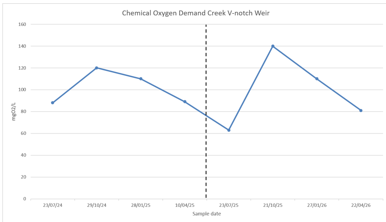
Figure 11 Chemical Oxygen Demand - Bypass Creek V-notch Weir
